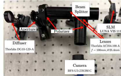
Fig. 6: Hardware prototype.
