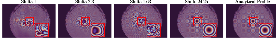
Fig. 7: Optical phase recovery of a biconvex lens ( f = 75 mm). Recovered phase under different shifts; the last column is the analytical thin-lens reference. Optimal co-prime shifts (24, 25) closely match the analytical rings (visible in the zoomed views), while non-optimal shifts introduce discontinuities and artifacts.
