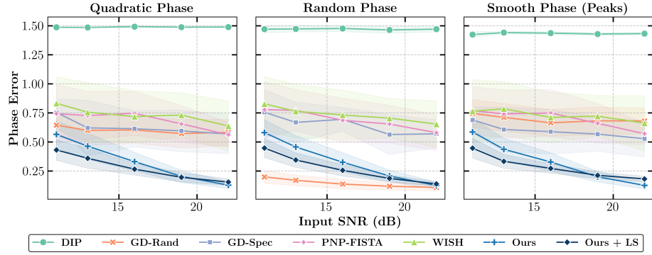
Fig. 5: Phase recovery performance across SNRs in simulations. Our method demonstrates consistent performance across all phase types, maintaining the lowest error in most settings and highly competitive results otherwise. Notably, least-squares refinement ( Ours + LS ) significantly improves reconstruction accuracy at low SNRs.
